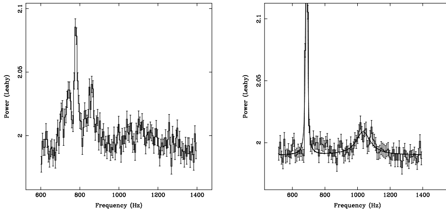
Figure 2. Left Panel: Average (standard) power spectrum of the same data shown in Figure 1. Right Panel: Shifted-and-averaged power spectrum of the same data.
